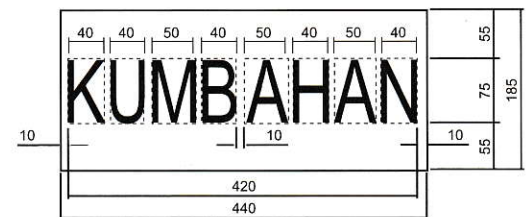
DETAIL '4' : EMBOSSED LOGO
