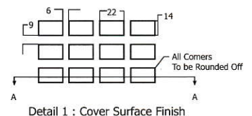
Detail 1 : Cover Surface Finish
